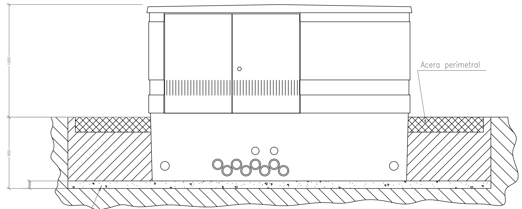
ALZADO PRINCIPAL
